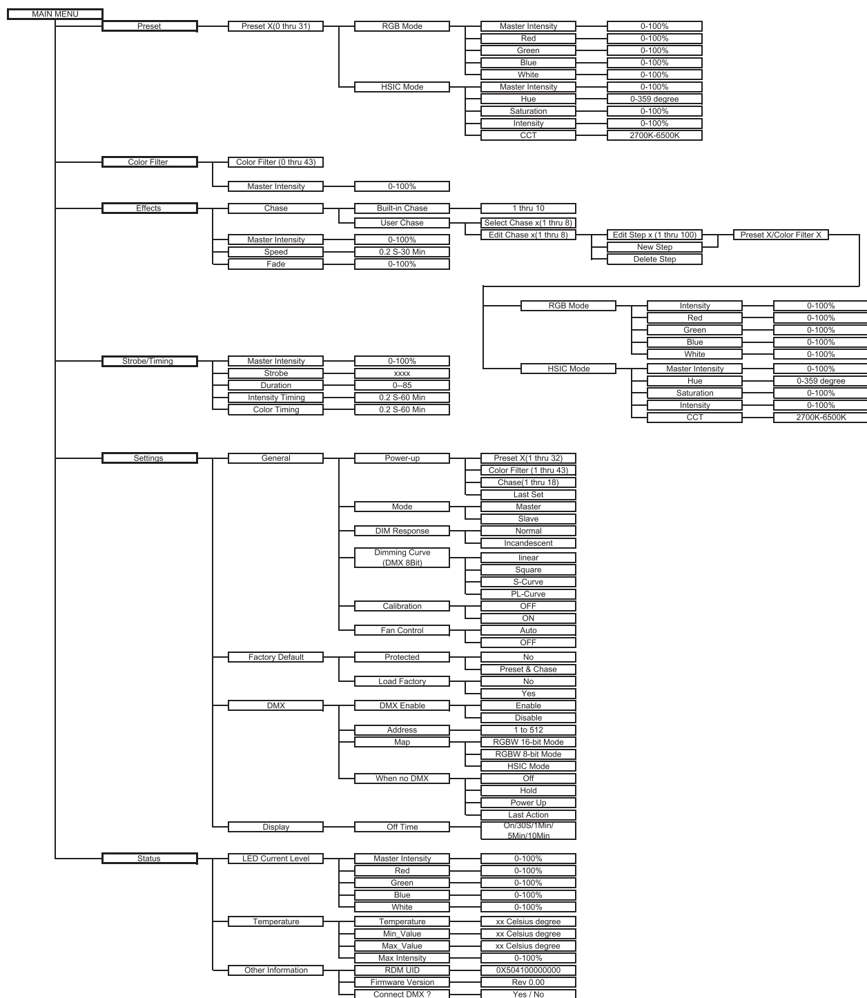
Figure 8: SL ePAR 180 LED Luminaire Menu Tree
